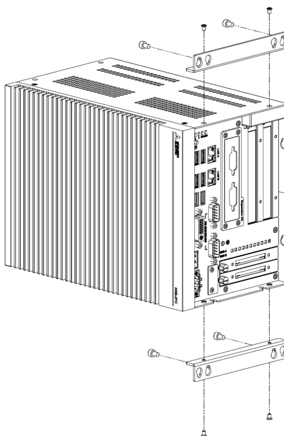
Figure 3.3 Enclosure Mount
