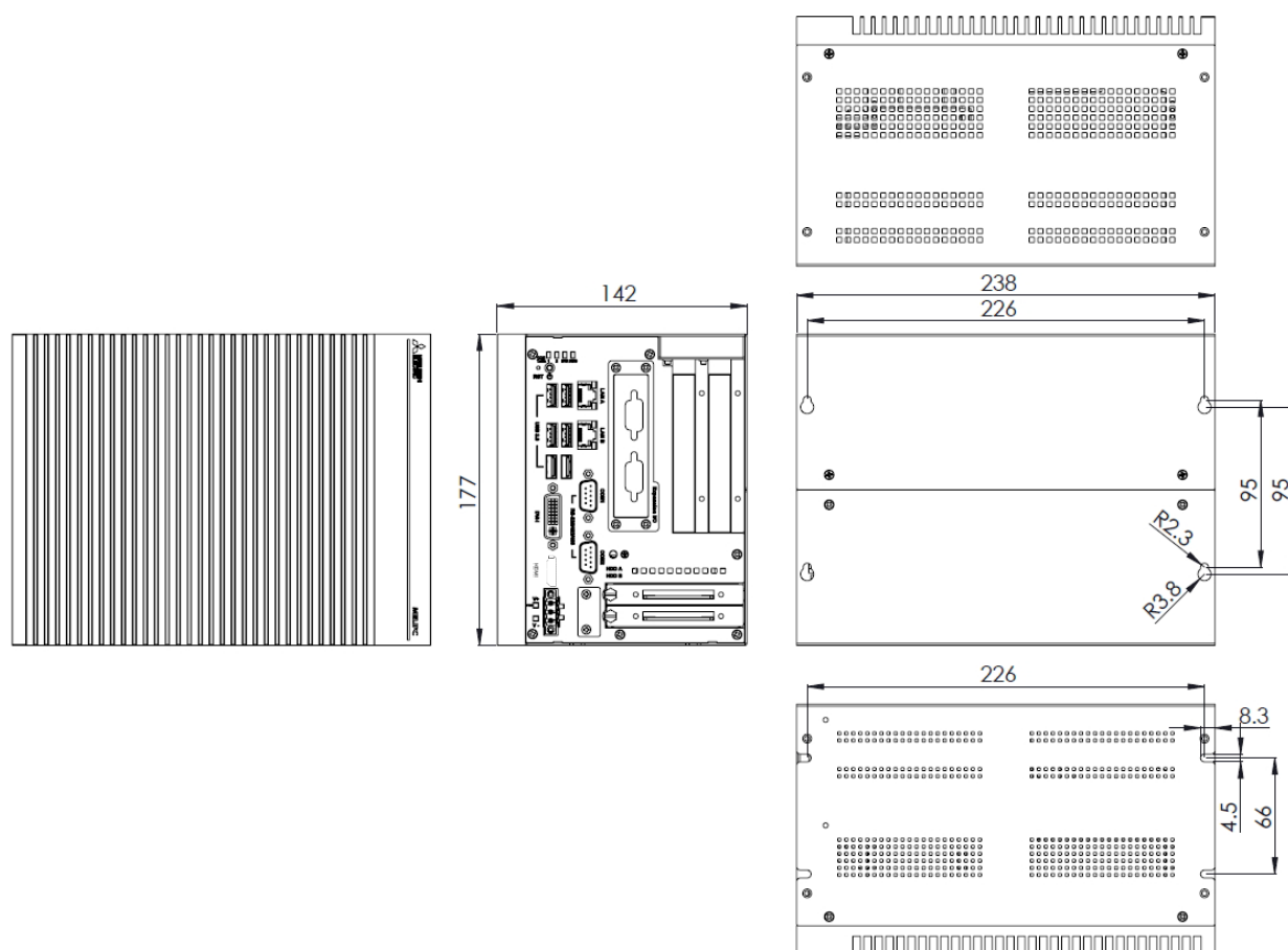
Figure 1.1 MI2012-W Dimensions
