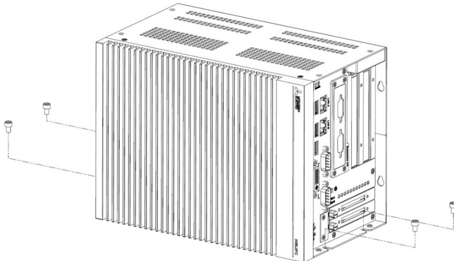
Figure 3.2 Stand Mount
