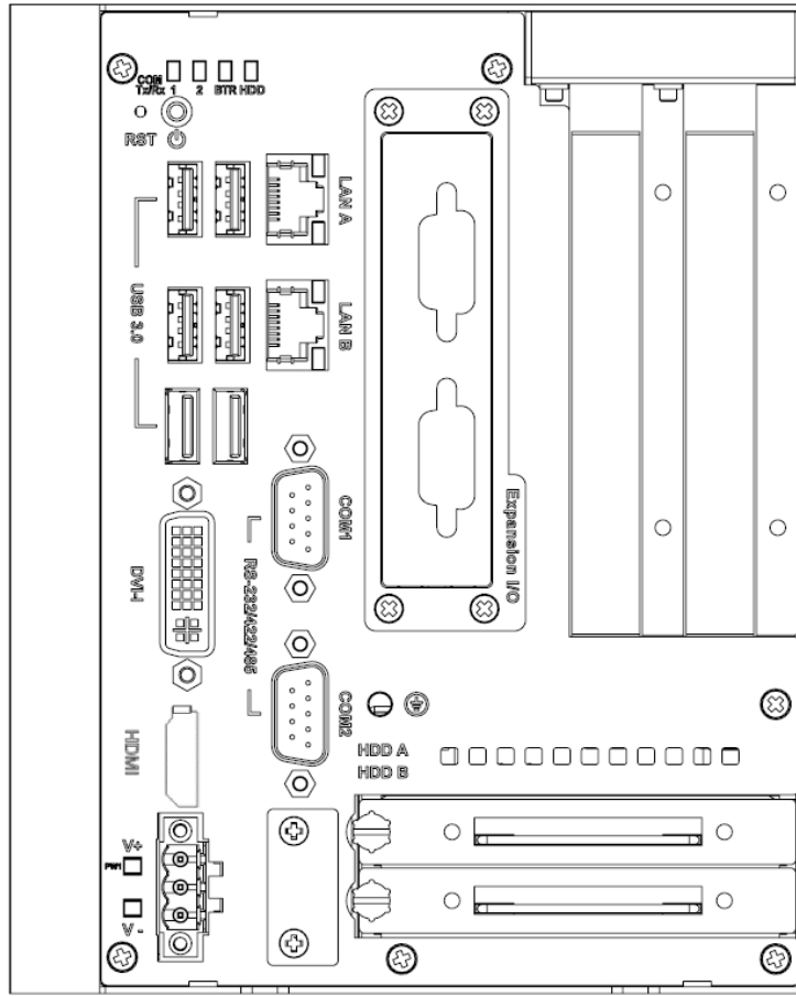
Figure 2.1 MI2012-W (Front View)
