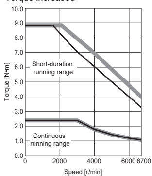
[HK-MT7M3W] Torque increased
