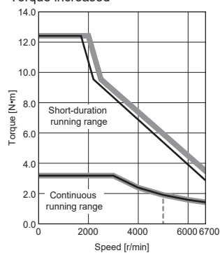
[HK-MT103W] Torque increased
