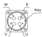
Power connector
