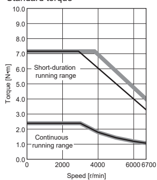
[HK-MT7M3W] Standard torque
