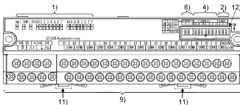
AJ65SBTB32-8 □ (Terminal block 8 point module, 3-wire input, 2-wire output)
