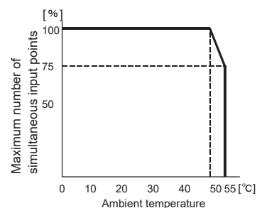
Derating curve (2)
