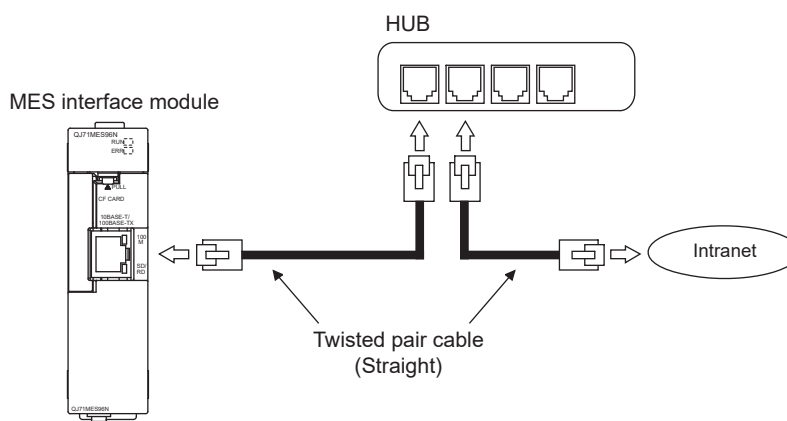
Figure 4.6 Wiring
