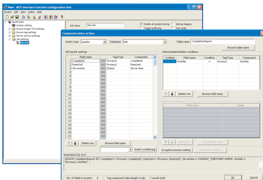
Figure 1.2 [MX MESInterface] - [MES interface function configuration tool]
