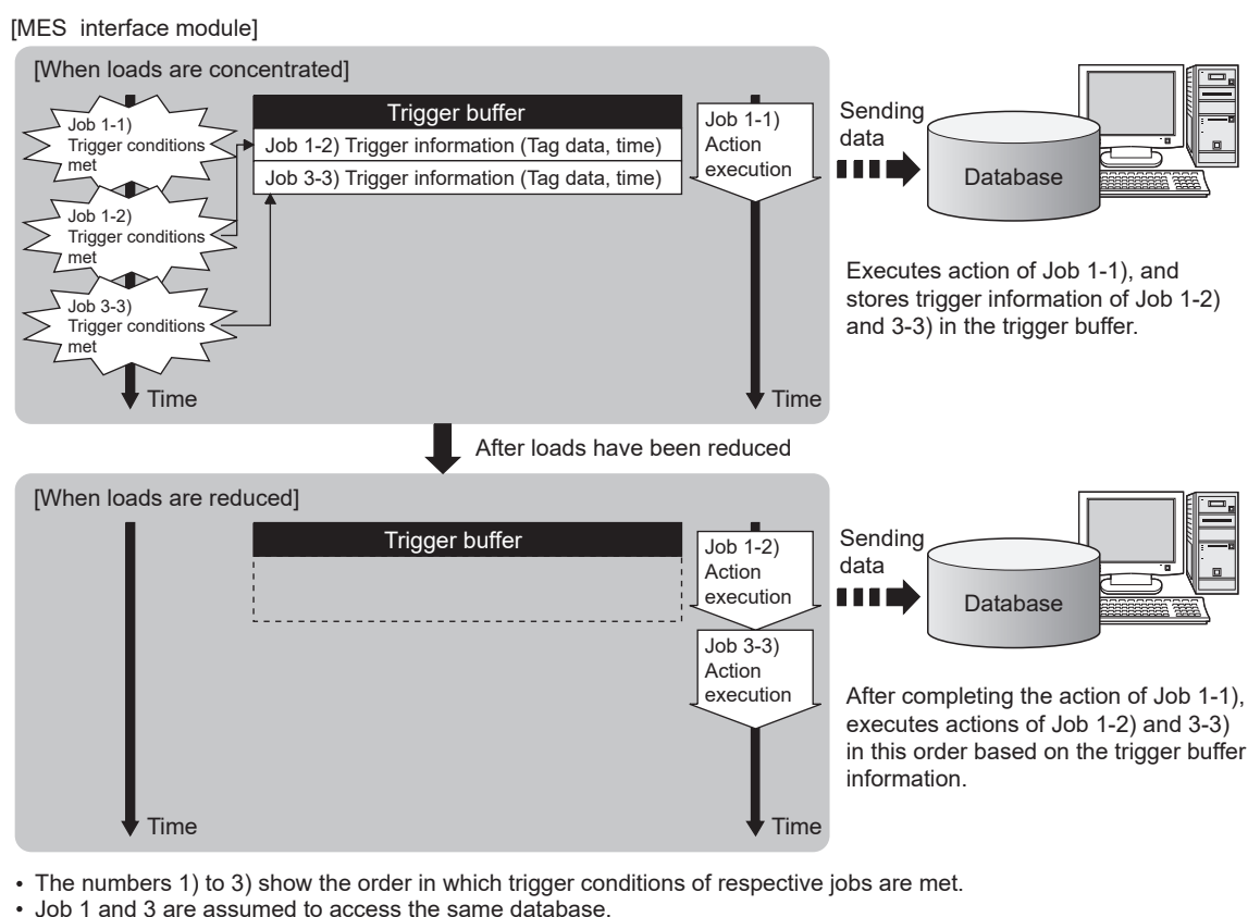
Figure 1.4 Data buffering in the case of load concentration
