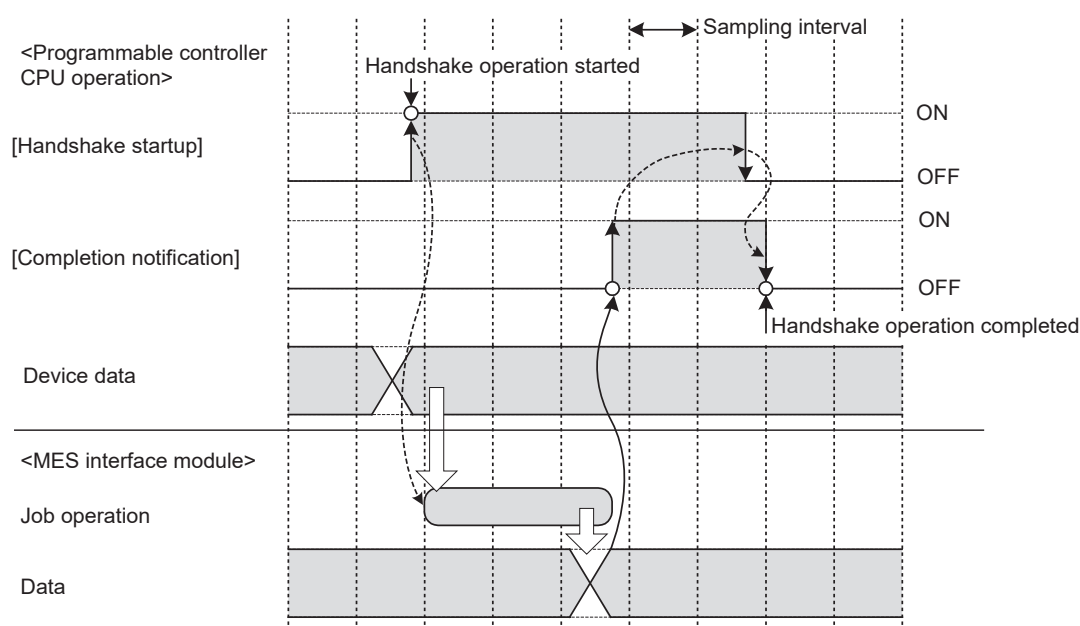
Figure 7.54 [Handshake operation]
